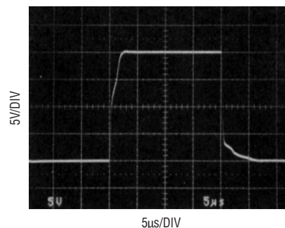
Pulse Response of Feedforward Compensation
